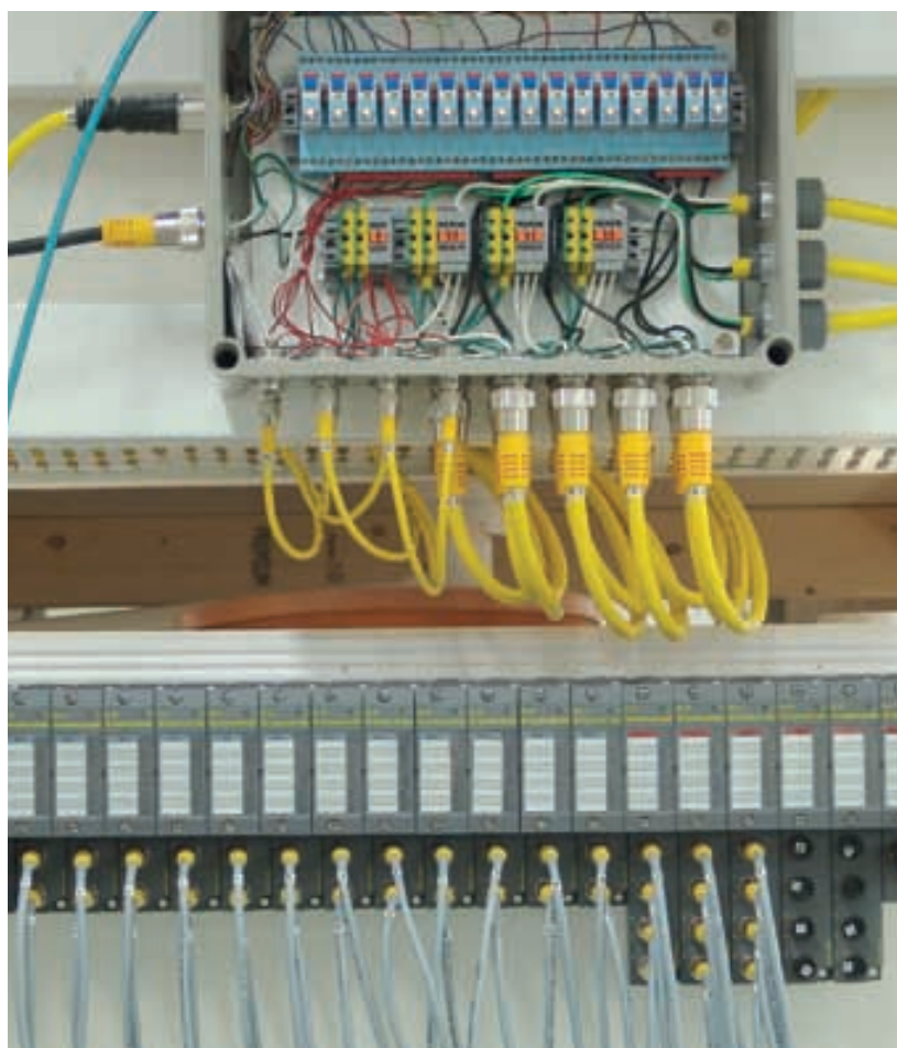
Flexible and reliable: The BL67 remote I/O system forwards measurement and control signals directly in the field
